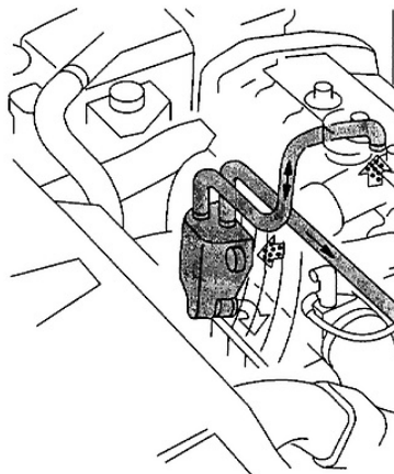
Figure 1. PCV Hose Modification
