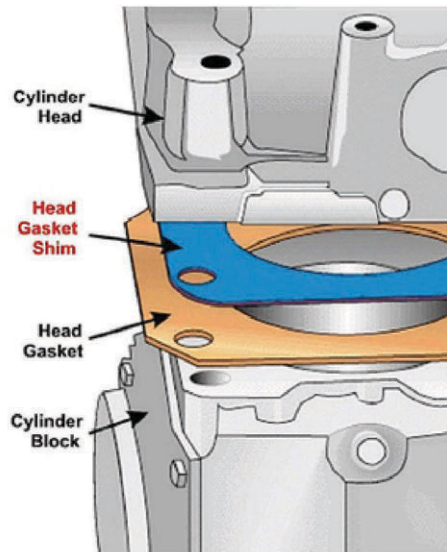
Figure 1. Typical Shim-Saver Installation
