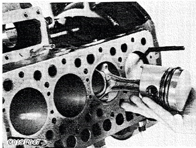
(A) Markings on the piston head
