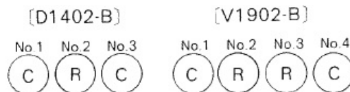
(A) Markings on the piston head
